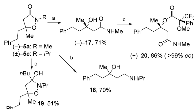
Scheme 7. Transformations of 5a and 5c ; synthesis of the tertiary alcohols: a) Raney-Ni, EtOH, 70 °C; b) Red-Al, THF/toluene (1:2), then zinc, AcOH/H 2 O (9:2); c) n BuLi, toluene, –78 °C to 10 °C; d) (S)-(+)- \alpha -methoxy- \alpha -(trifluoromethyl)phenylacetyl chloride, Et 3 N, CH 2 Cl 2 , 40 °C. Red-Al = sodium bis(2-methoxyethoxy)aluminumhydride.
