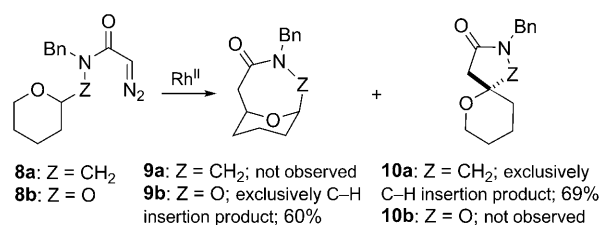
Scheme 5. [{Rh(OAc) 2 }] 2 -catalyzed reaction of tetrahydro-2H-pyran-2-yl ( 8a ) and tetrahydro-2H-pyran-2-yl-oxy ( 8b ) diazo analogues. The reaction conditions are the same as those indicated in the Table 2. In the case of 8a , a minor product that was derived from the Buchner reaction was observed; Bn = benzyl.
